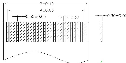
RECOMMENDED FPC DIMENSION
